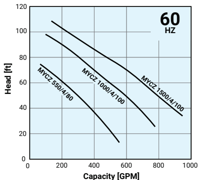
MYCZ: Chopper (Stock)
