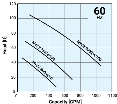
MYCZ: Chopper (Non-Stock)
