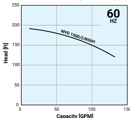
MYG: Grinder (Non-Stock)
