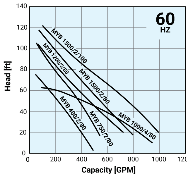
MYB: Open Channel (Non-Stock)
