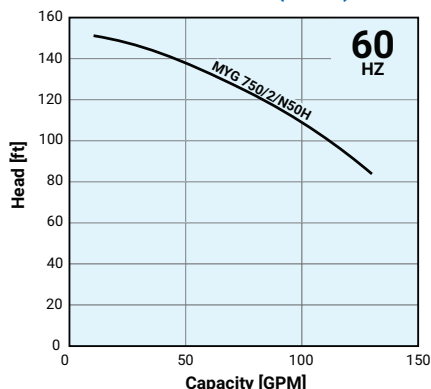
MYG: Grinder (Stock)
